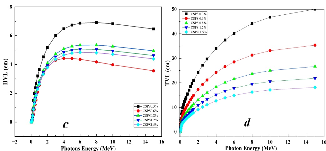
Figure 3: (c & d) HVL and TVL of 20\text{CaSO}_4 + (10-x) \text{P}_2\text{O}_3 - \text{Sm}_2\text{O}_3 glass systems.
