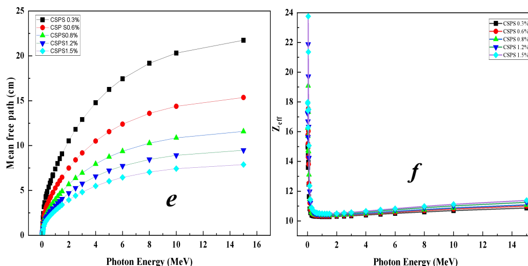
Figure 4: (e & f) MFP and Z_{\text{eff}} of 20\text{CaSO}_4 + (10-x) \text{P}_2\text{O}_3 - \text{Sm}_2\text{O}_3 glass systems.
